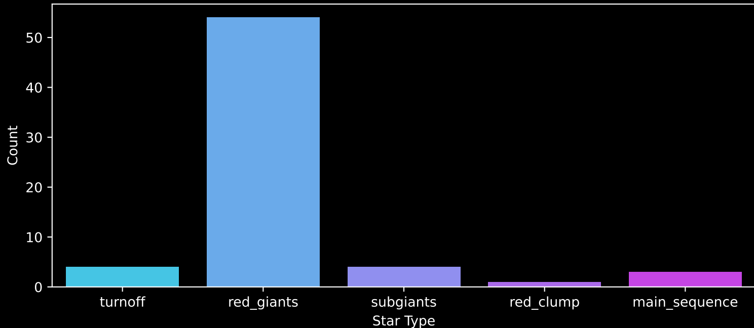
APOGEE DR17 Field: [303-45-O] Count plot of Star Type
