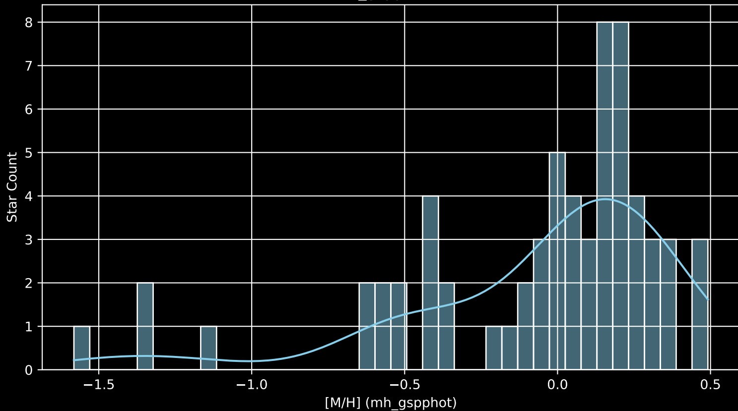
APOGEE DR17 Field: [303-45-O [M/H] (mh_gspphot) (n= 64)
