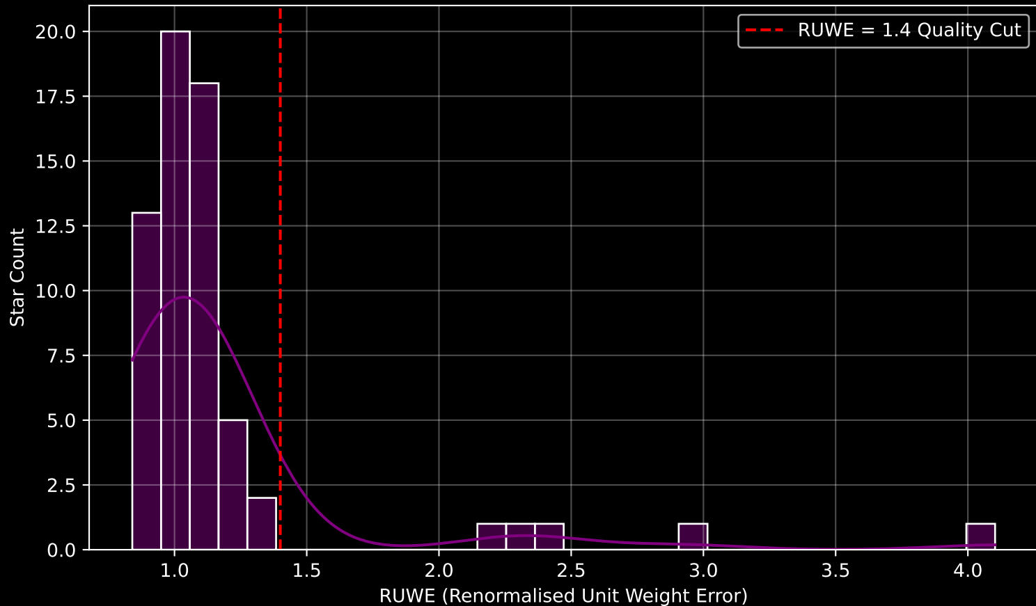
GAPOGEE DR17 Field [303-45-O] RUWE Distribution (n= 63)
