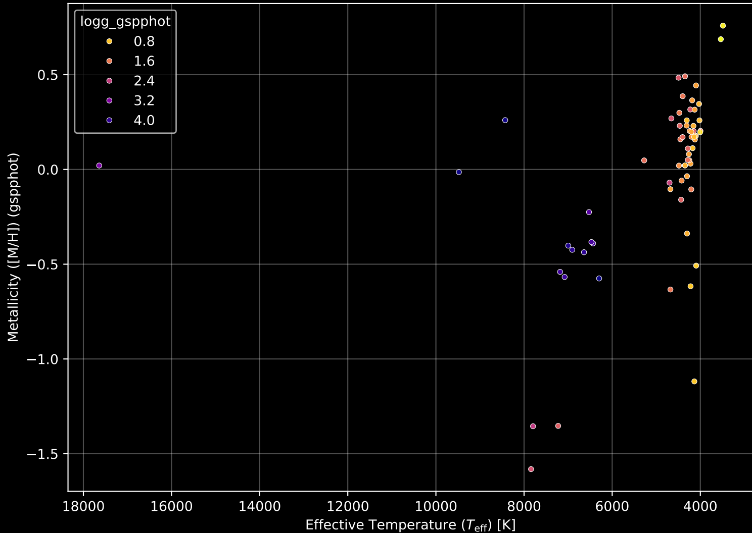
APOGEE DR17 Field: [303-45-O] Stellar Population Parameters (n= 66)
