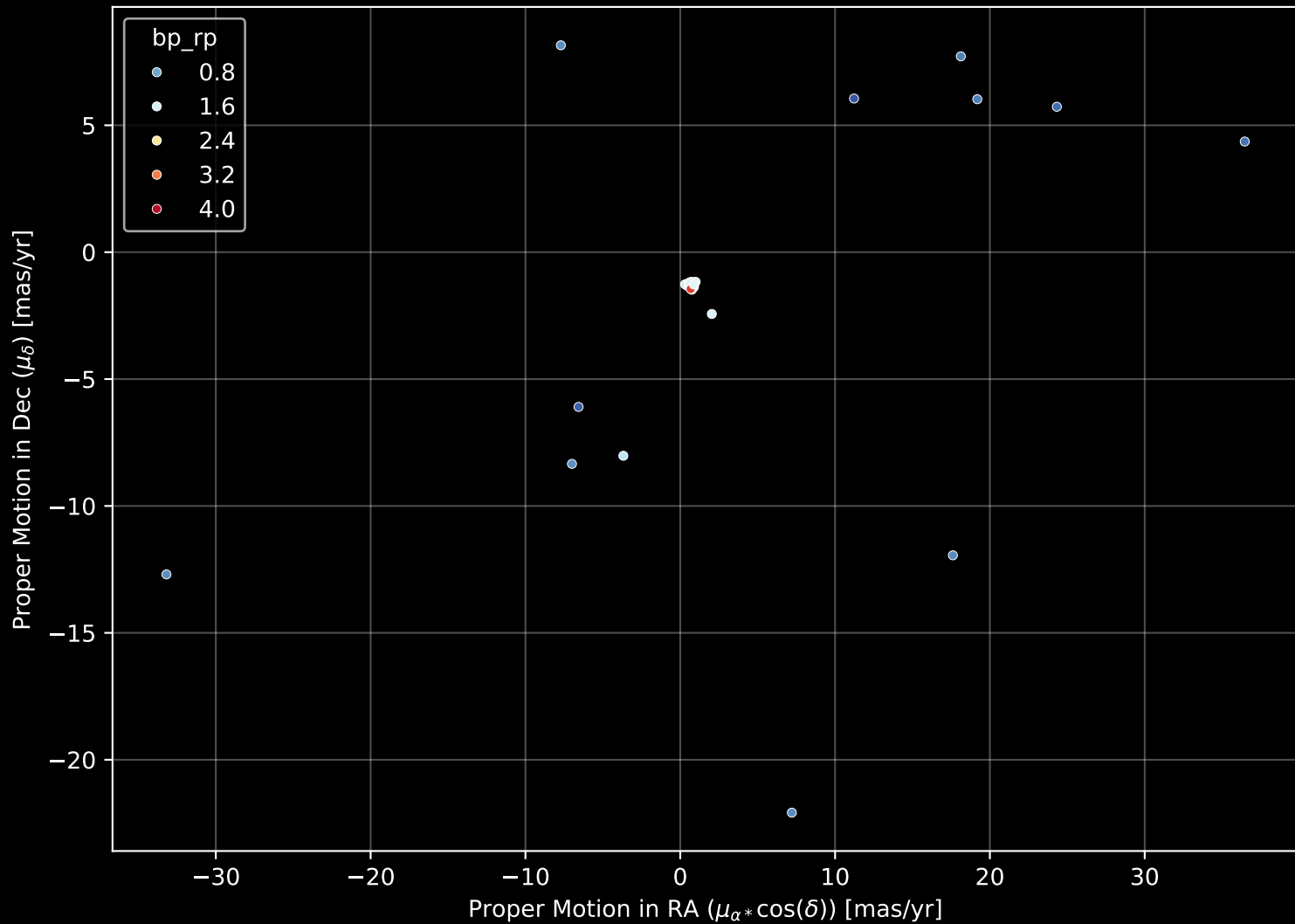
APOGEE DR17 Field: [303-45-O] Proper Motion Diagram (n= 66)
