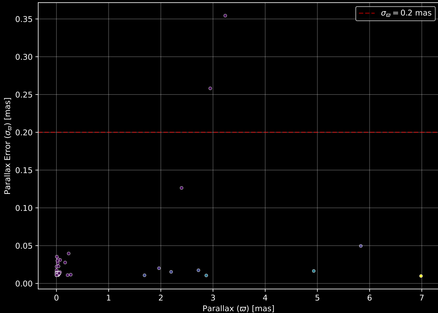
APOGEE DR17 Field: [303-45-O] Parallax Quality (n= 66)
